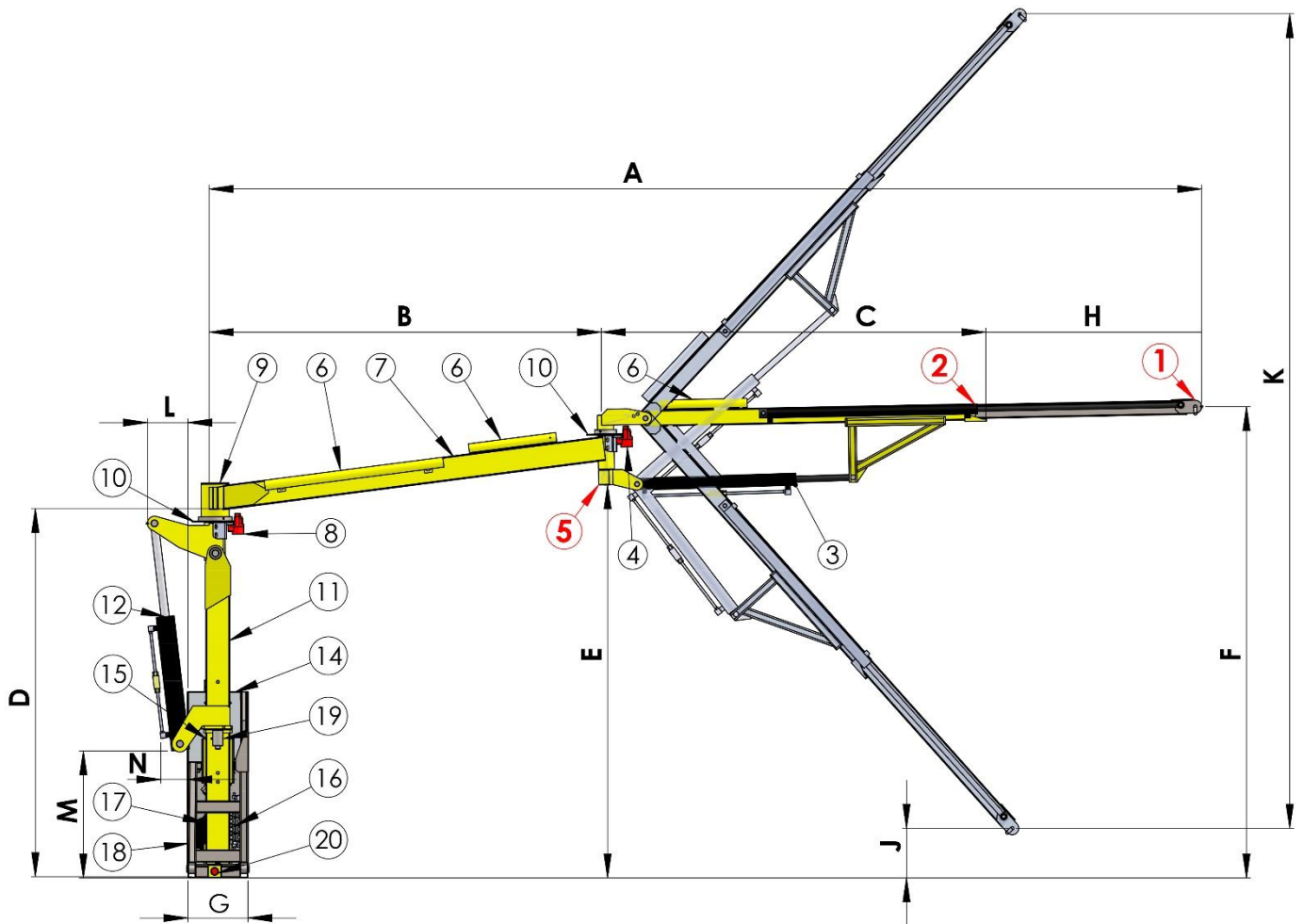
Figure 2. Scheme crane
